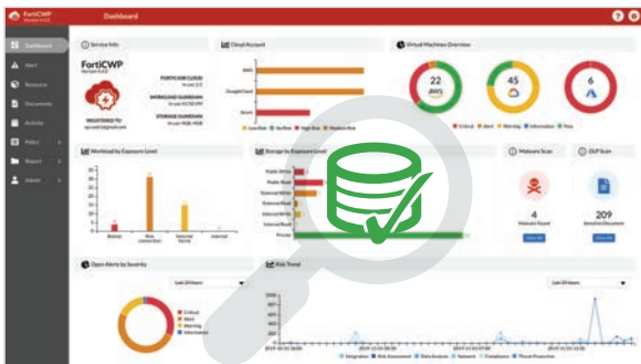
FortiCWP
